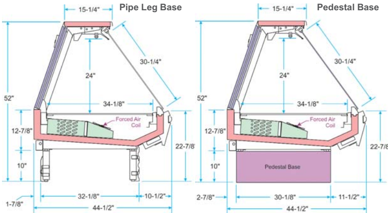
Pipe Leg Base
