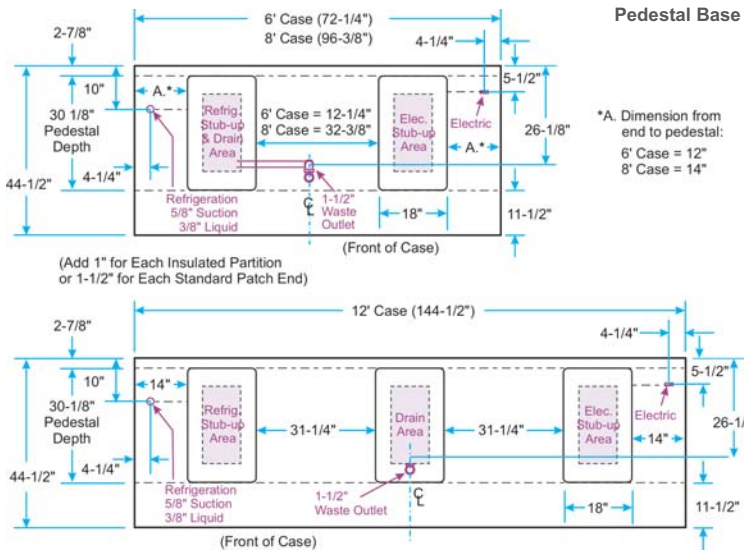
Pedestal Base
